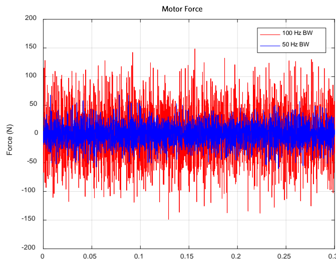
Figure 5. Motor force for 50 Hz vs. 100 Hz Bandwidth
