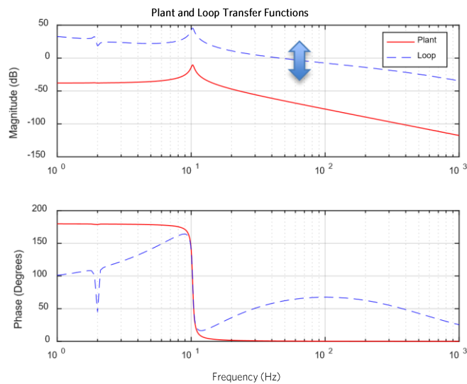
Figure 4. Plant and Loop Transfer Functions
