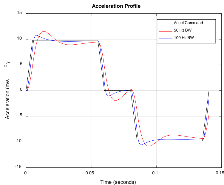
Figure 2 Motion Trajectory (Black - Commanded, Red - 50 Hz, Green - 100 Hz)
