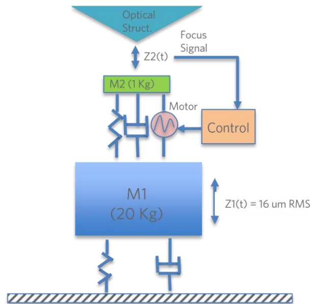
Figure 3 Simple Disturbance Tracking System
